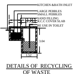
DETAILS OF RECYCLING OF WASTE
