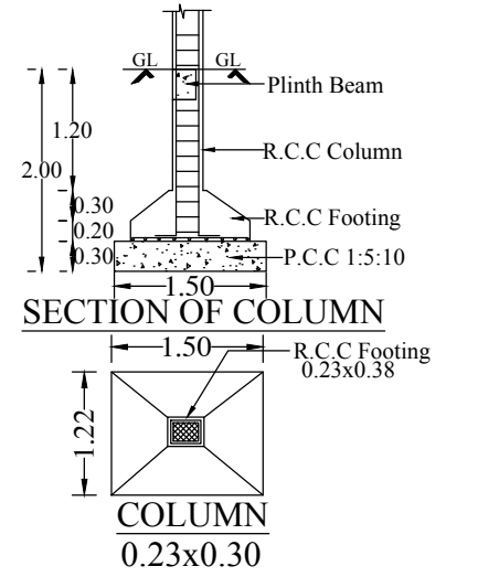
SECTION OF COLUMN
