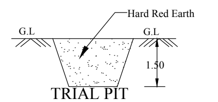
TRIAL PIT
