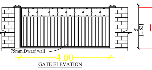
GATE ELEVATION
