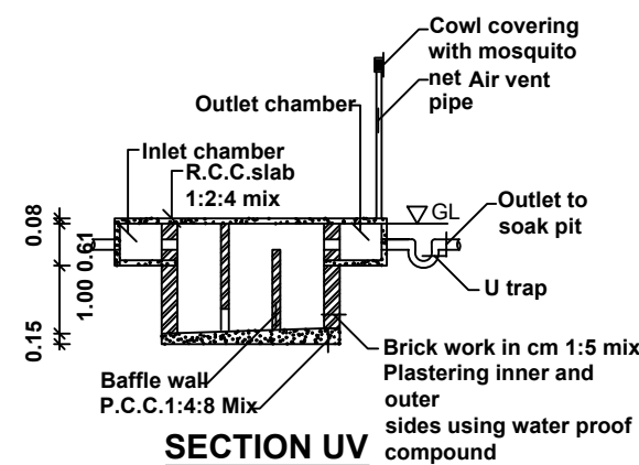
SECTION UV
