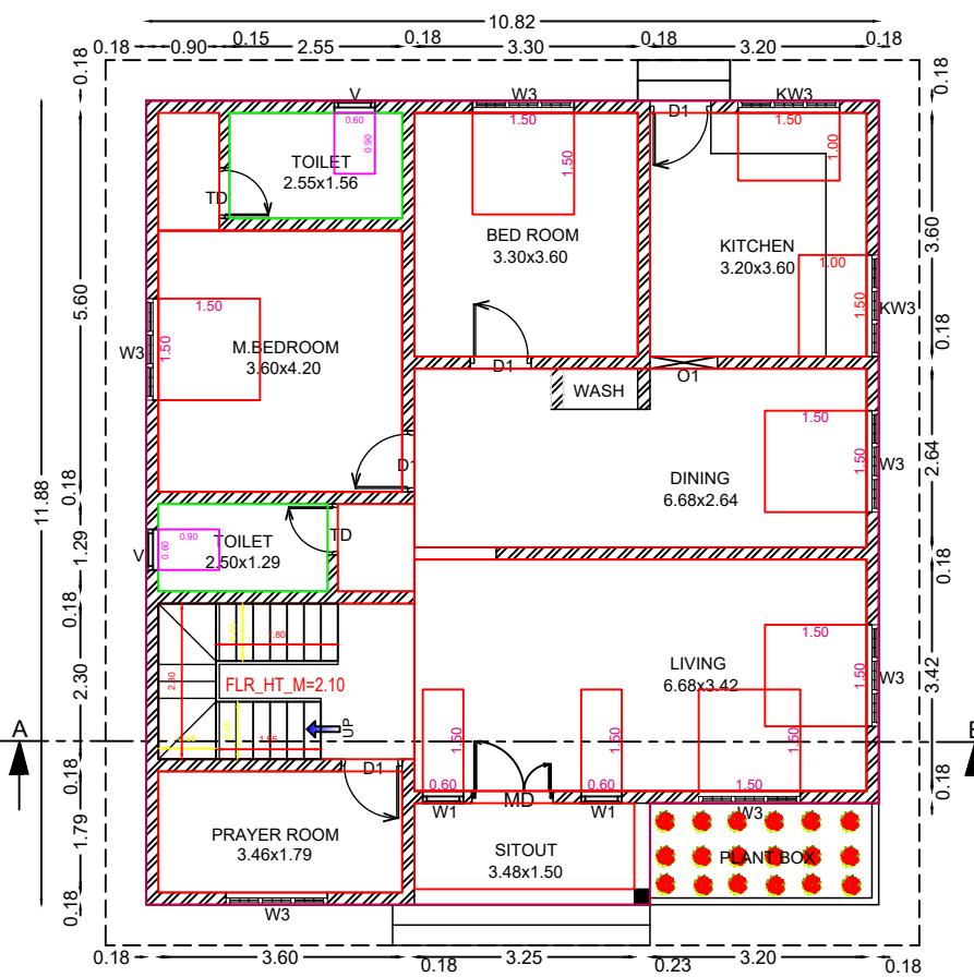
GROUND FLOOR PLAN BUILTUP AREA = 123.5 m 2 (1328.86 sq.ft)
