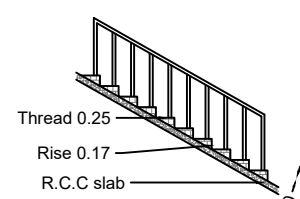
STAIRCASE DETAIL
