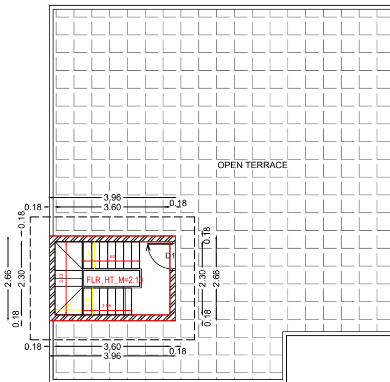
FIRST FLOOR PLAN BUILTUP AREA = 10.5 m 2 (112.98 sq.ft)
