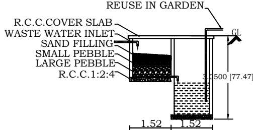
RECYCLING OF WASTE WATER
