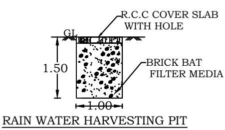
RAIN WATER HARVESTING PIT
