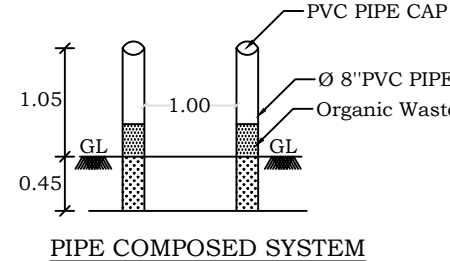
PIPE COMPOSED SYSTEM
