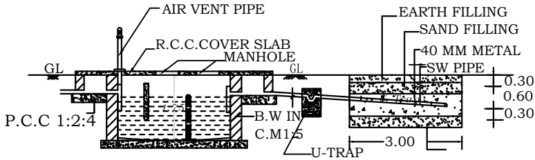
SECTION SECTION OF DISPERSION TRENCH
