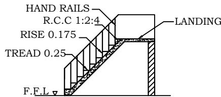
STAIR CASE DETAIL
