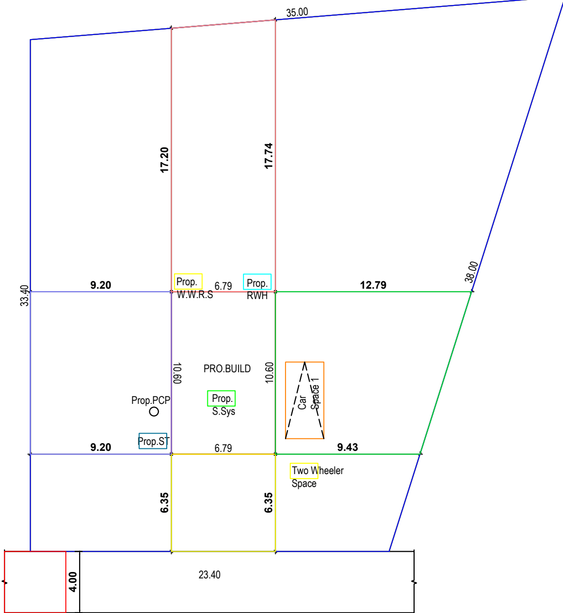
SITE PLAN
