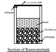
Section of Rainwater tank
