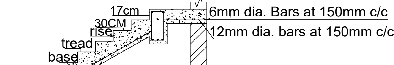
SECTION OF STAIRCASE
