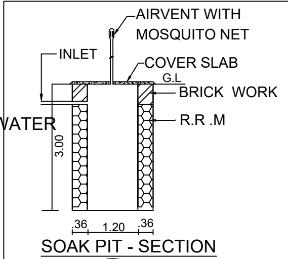
SOAK PIT - SECTION
