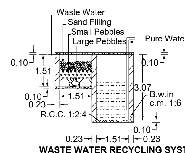
0.23-1.5-0.23 WASTE WATER RECYCLING SYSTEM
