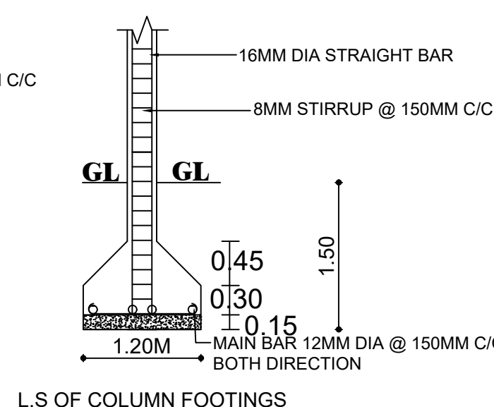
L.S OF COLUMN FOOTINGS
