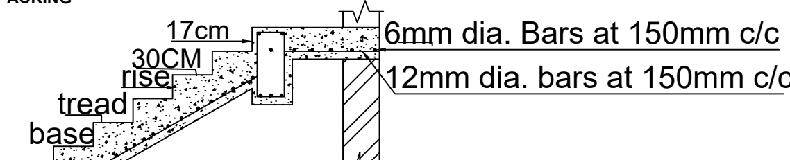
SECTION OF STAIRCASE
