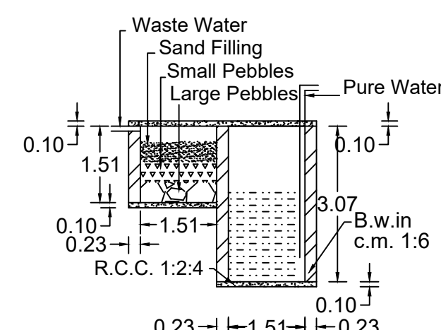
WASTE WATER RECYCLING SYSTEM
