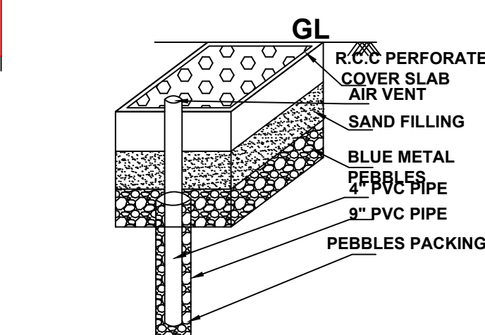
PERCOLATION BORE PIT
