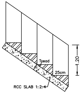
STAIR DETAILS
