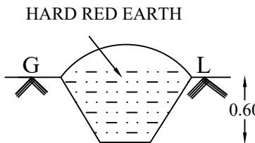
TRIAL PIT SECTION
