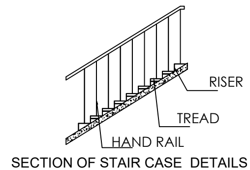
SECTION OF STAIR CASE DETAILS
