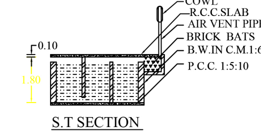
WASTE TRASH PIT
