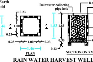
RAIN WATER HARVEST WELL
