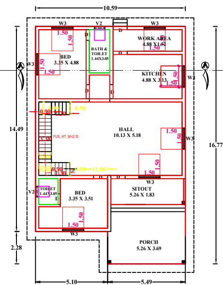
PLAN (GROUND FLOOR)
