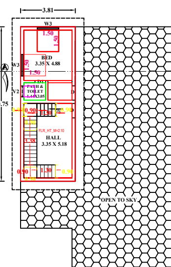
PLAN (FIRST FLOOR)
