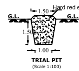
TRIAL PIT (Scale 1:100)
