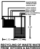
RECYCLING OF WASTE WATER FROM KITCHEN & BATHROOM
