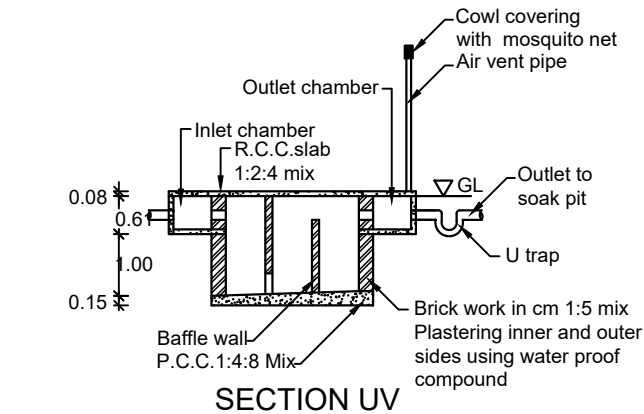
SECTION UV
