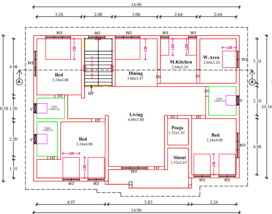
GROUND FLOOR PLAN AREA:160.12M2(1723.51SQ.FT)
