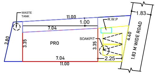
SITE PLAN (SCALE 1:100)
