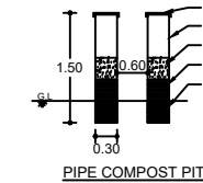
PIPE COMPOST PIT
