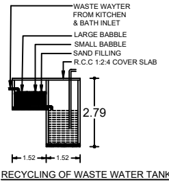
RECYCLING OF WASTE WATER TANK
