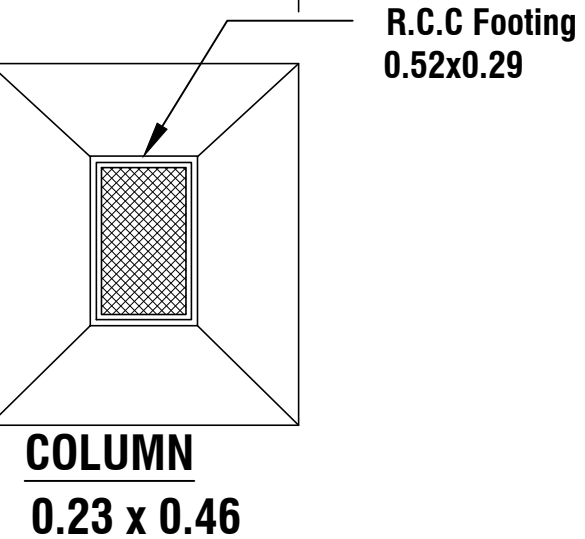
SECTION OF COLUMN
