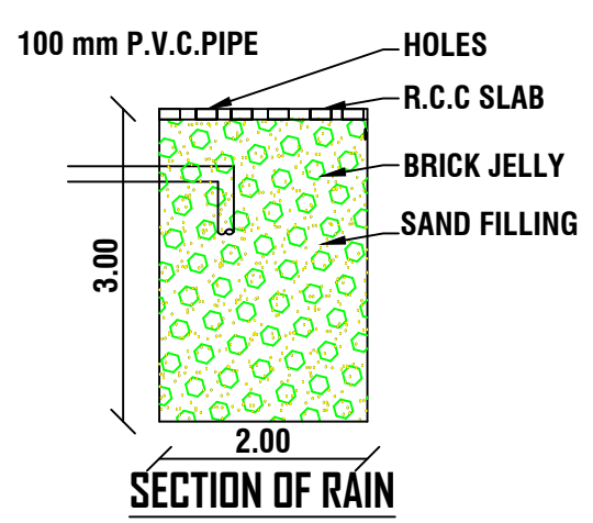
Rain water pit
