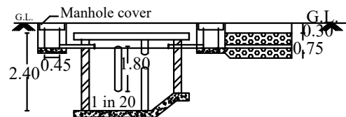
DETAILS OF SEPTIC TANK
