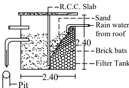
Rain Water Storage
