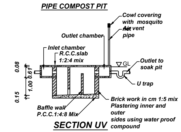
PIPE COMPOST PIT
