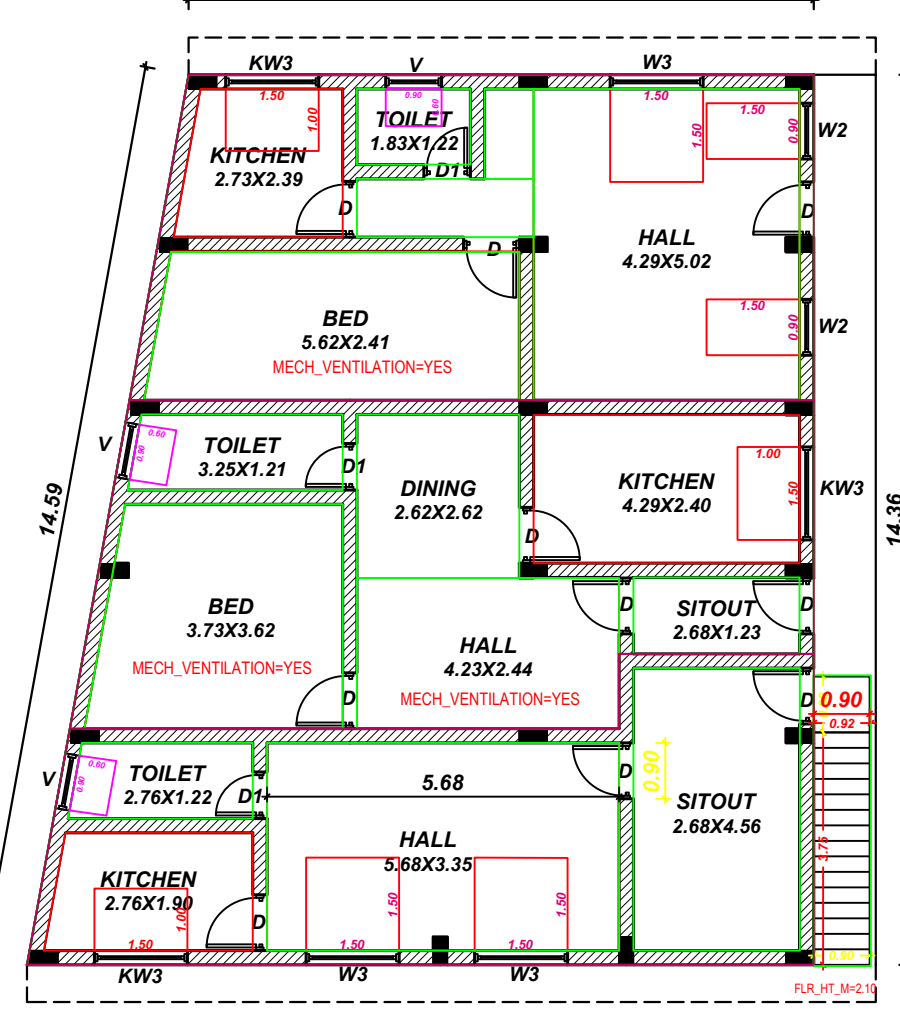
FIRST FLOOR PLAN PROPOSED BUILDING
