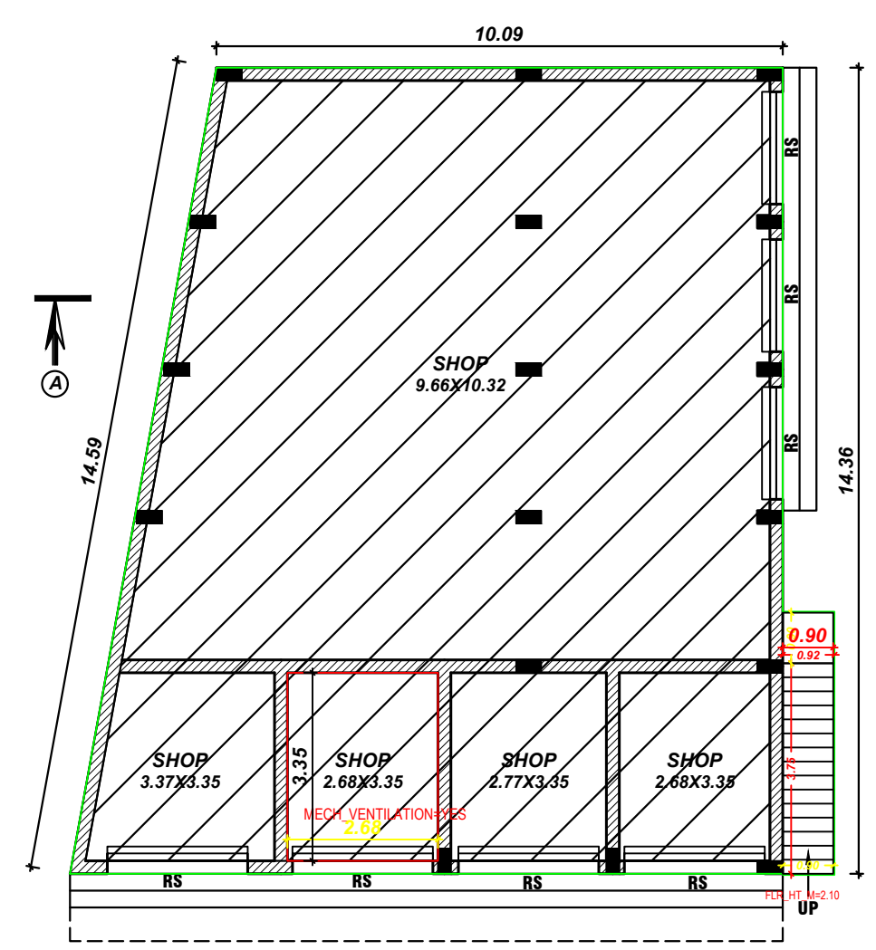
GROUND FLOOR PLAN EXISTING BUILDING
