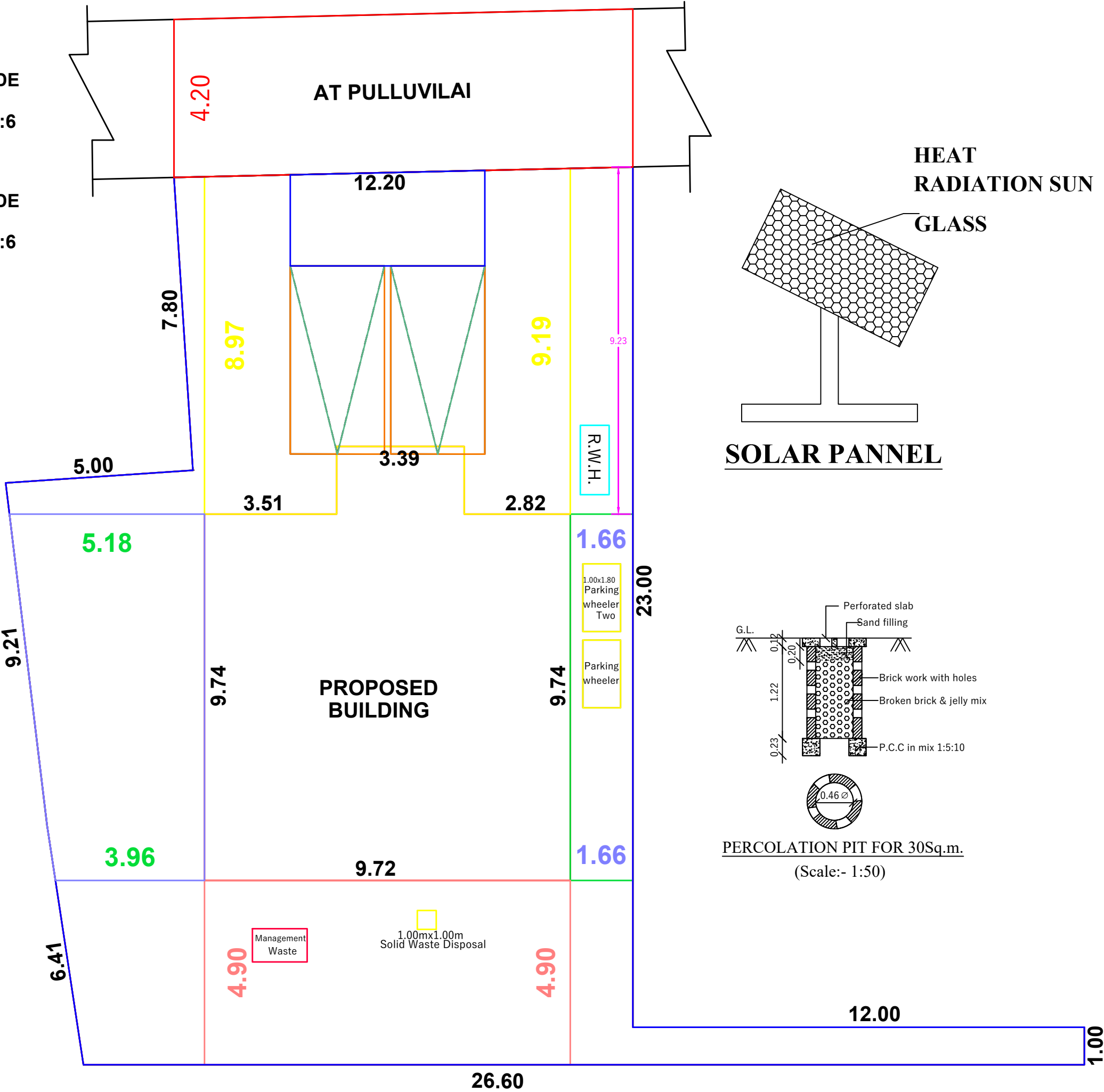
SITE PLAN
