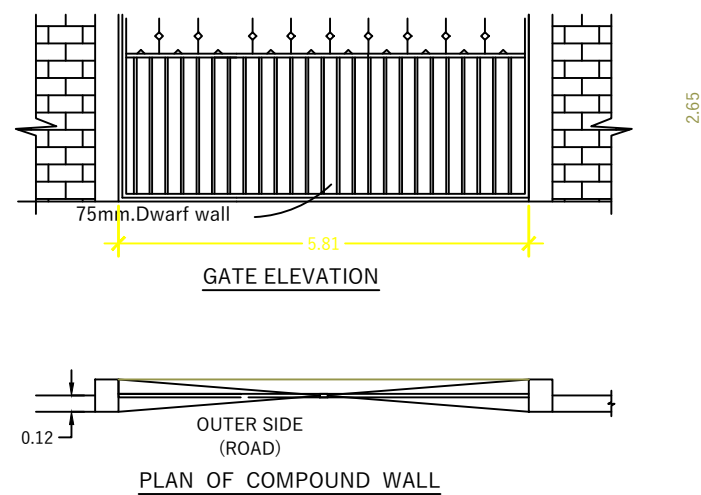
PLAN OF COMPOUND WALL
