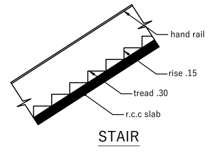
STAIR
