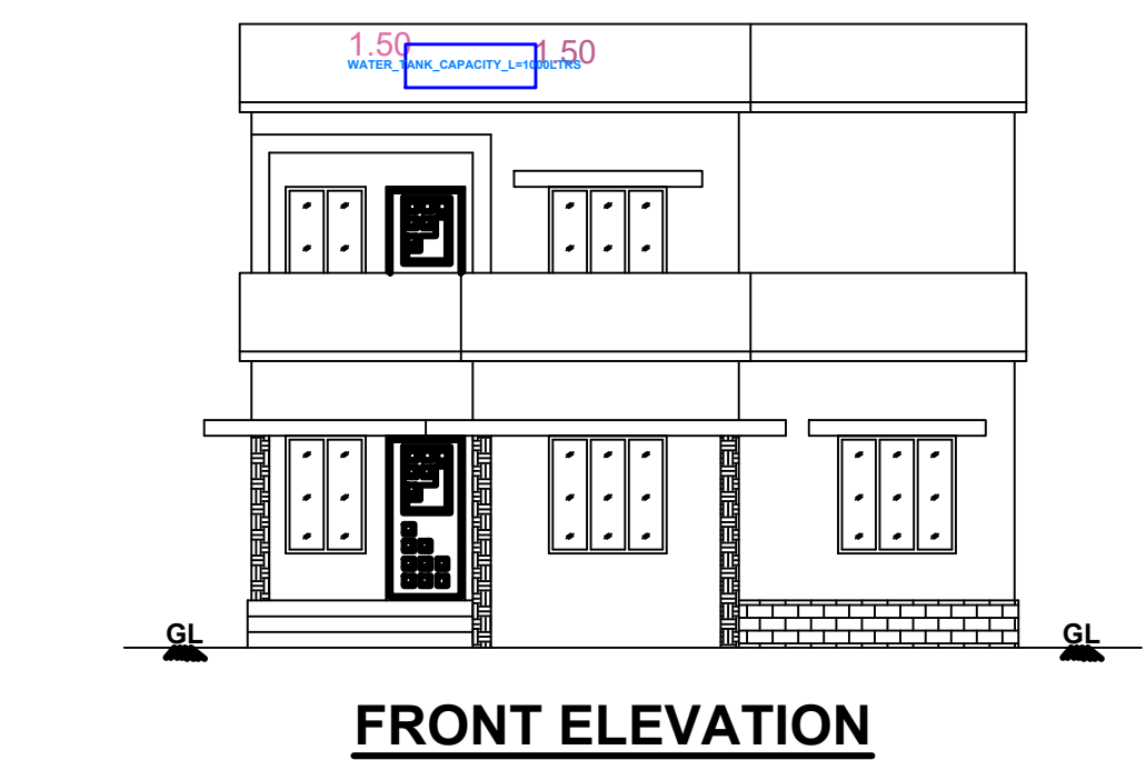
FRONT ELEVATION
