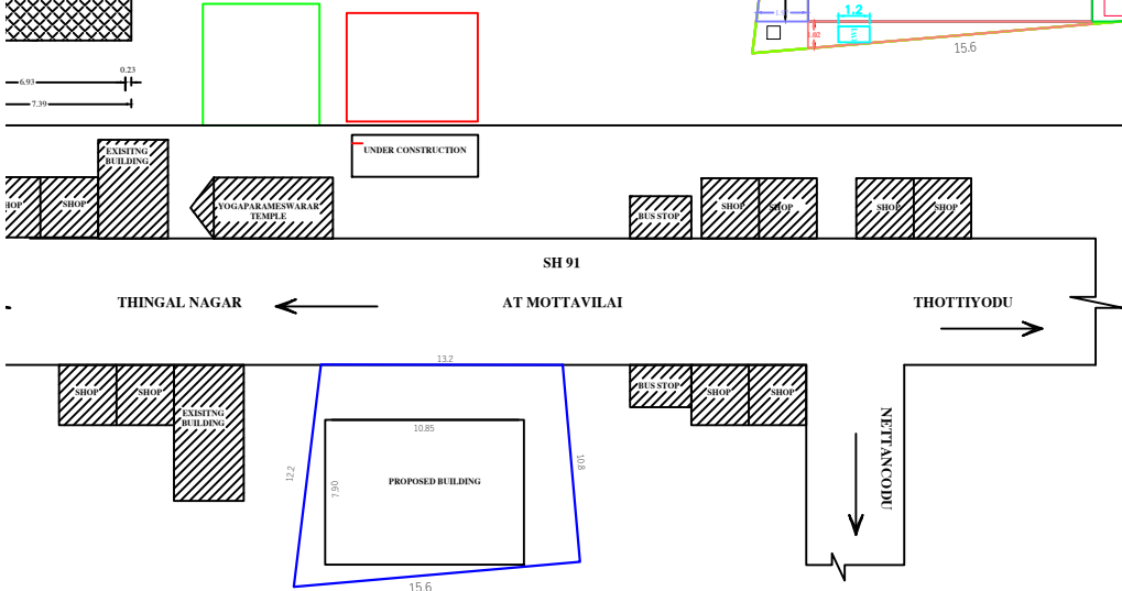
KEY PLAN
