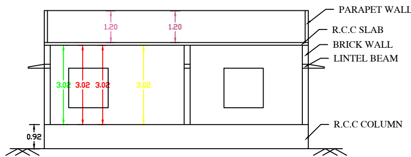
SECTION AT X-X'
