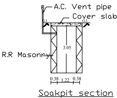
Soakpit section
