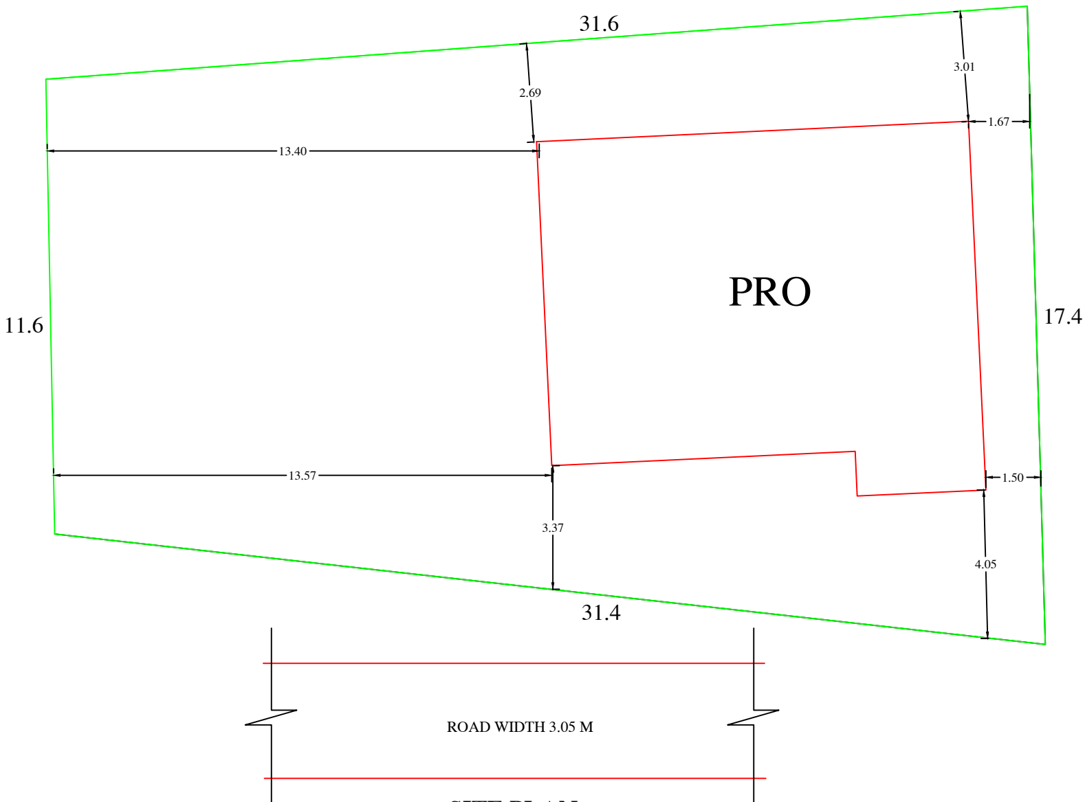
SITE PLAN
