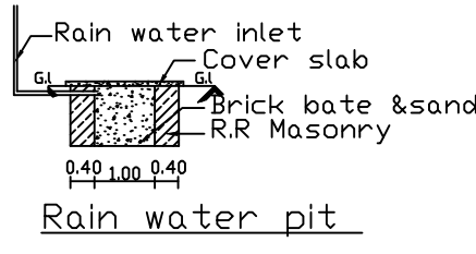
Rain water pit
