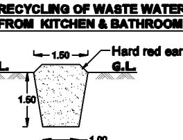
RECYCLING OF WASTE WATER FROM KITCHEN & BATHROOM
