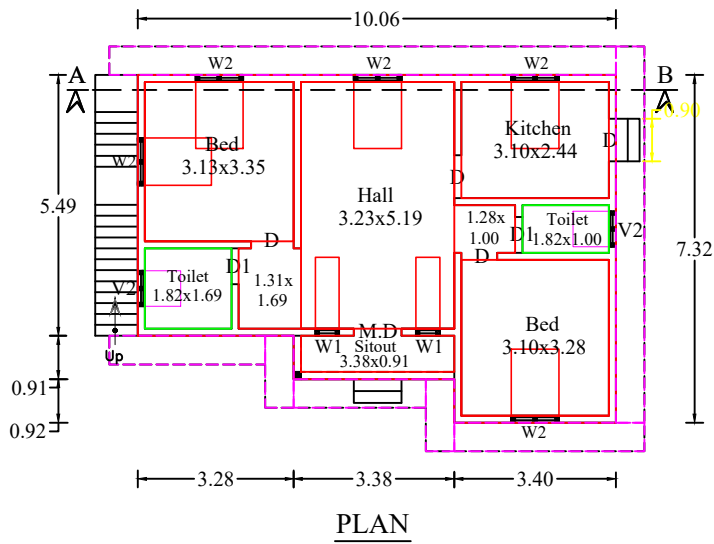
PLAN
