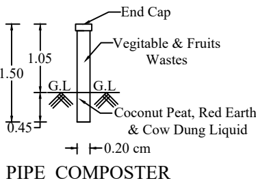
PIPE COMPOSTER
