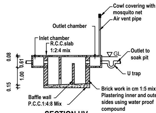
SECTION UV
