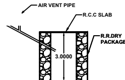
SECTION OF SOAKPIT
