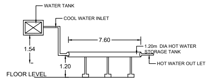
SOLAR WATER HEATING SYSTEM(S.W.H.S. DETAILS)
