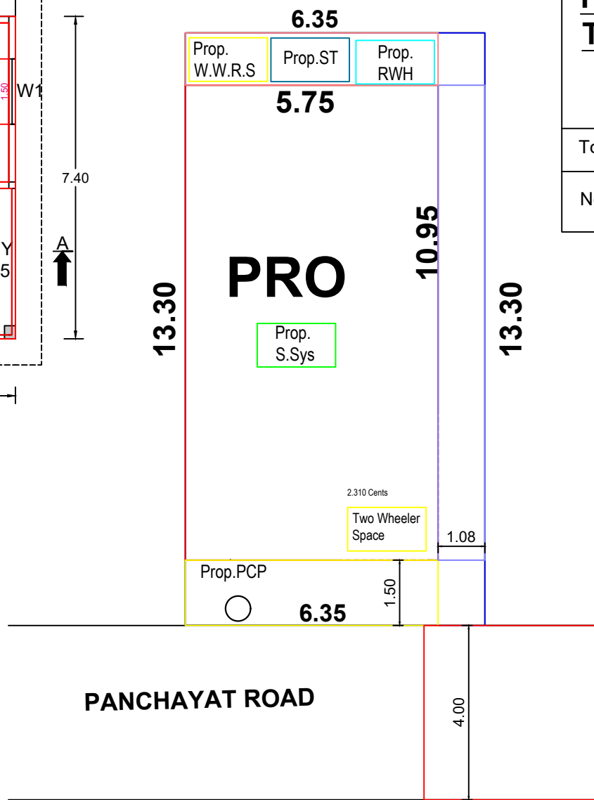
SITE PLAN SCALE : 1 CM = 1 M
