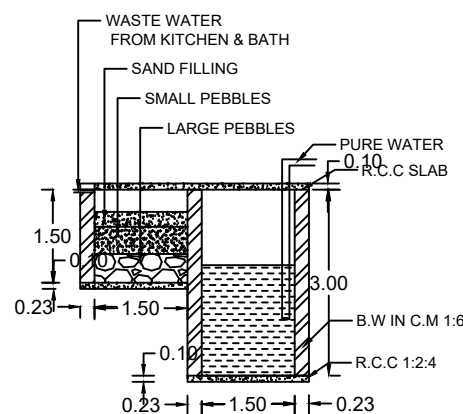
WASTE WATER RECYCLING SYSTEM
