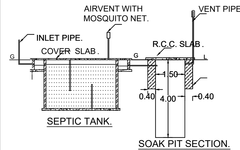
SOAK PIT SECTION.
