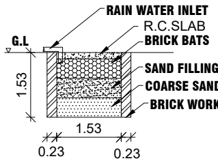
RAIN WATER HARVESTING PIT RWH_CAPACITY_L=5000LTRS
