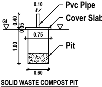
SOLID WASTE COMPOST PIT
