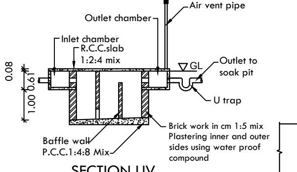
SECTION UV
