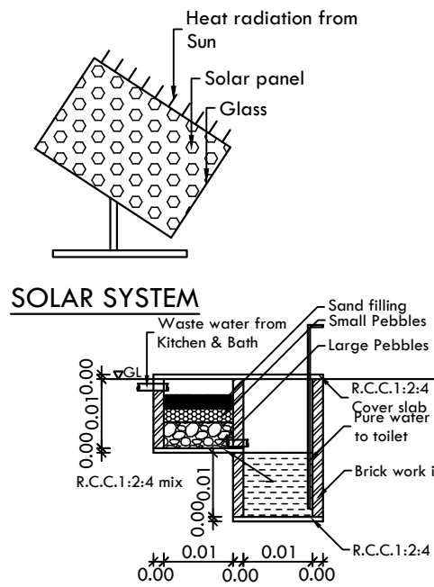
WASTE WATER RECYCLING SYSTEM
