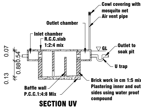
SECTION UV
