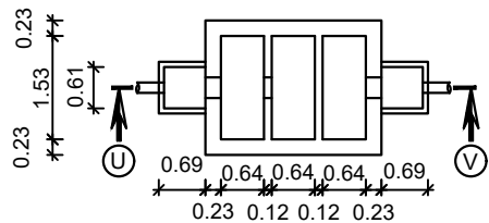
SECTION UV
