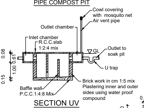
SECTION UV
