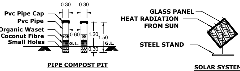
SOLAR SYSTEM
