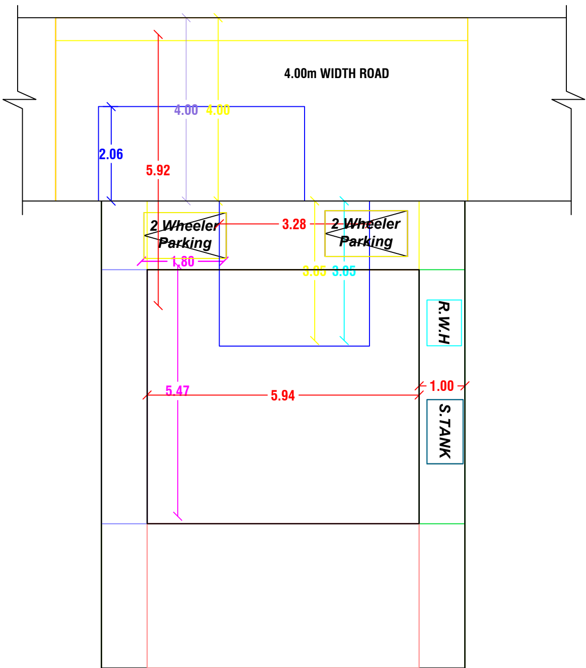
SITE PLAN
