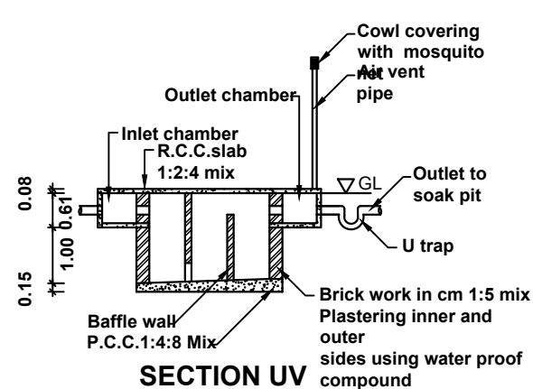
SECTION UV
