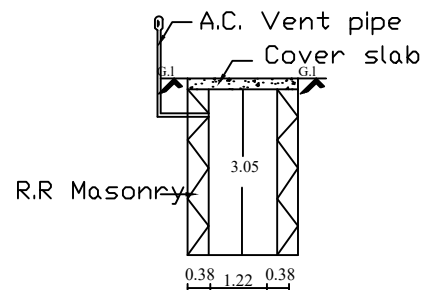
Soakpit section
