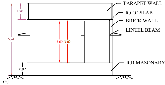
SECTION AT X-X'
