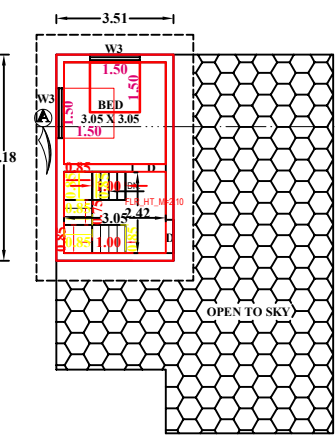
PLAN (FIRST FLOOR)
