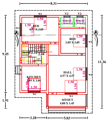
PLAN (GROUND FLOOR)
