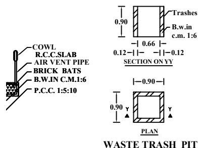
WASTE TRASH PIT
