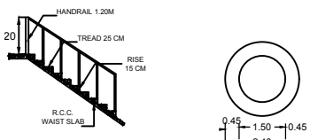
STAIRCASE DETAILS
