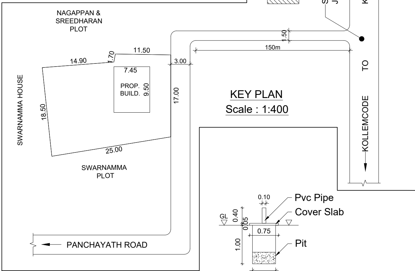
RAIN WATER HARVESTING PIT
