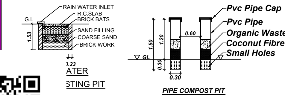
PIPE COMPOST PIT
