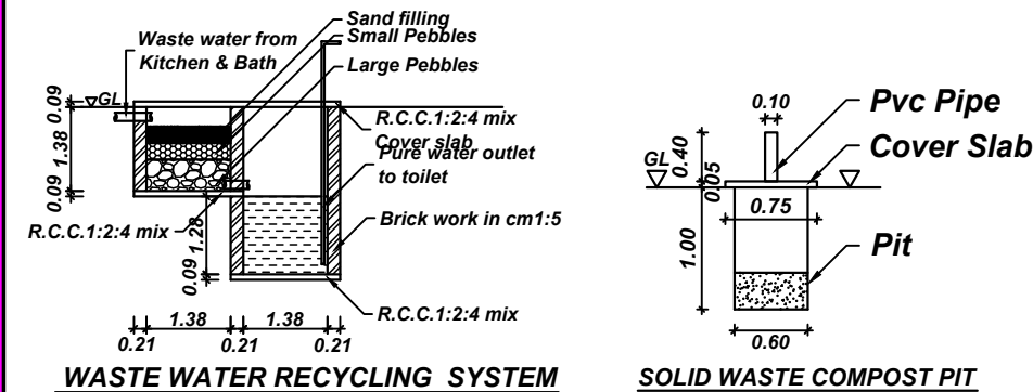
WASTE WATER RECYCLING SYSTEM
