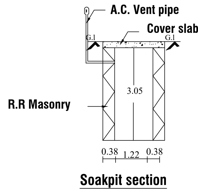
Soakpit section
