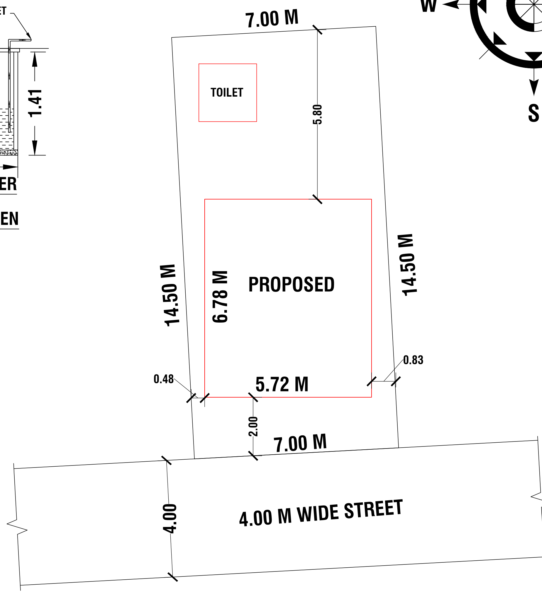
SITE PLAN
