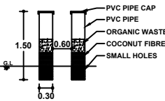
PIPE COMPOST PIT
