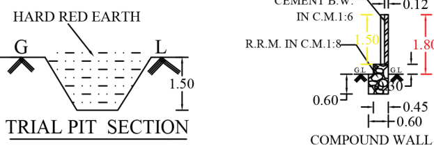
COMPOUND WALL
