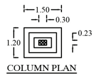
COLUMN PLAN
