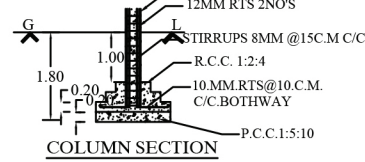
COLUMN SECTION
