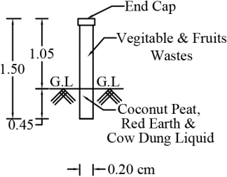
PIPE COMPOSTER
