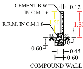
COMPOUND WALL
