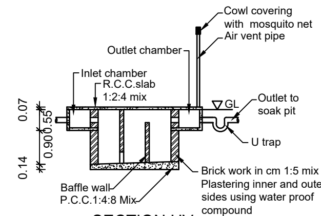
SECTION UV
