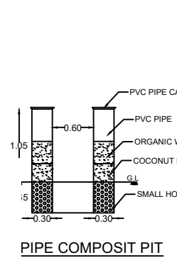
PIPE COMPOSIT PIT
