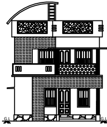
BLOCK-01 ELEVATION @ EAST SIDE
