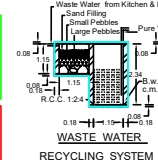
WASTE WATER RECYCLING SYSTEM
