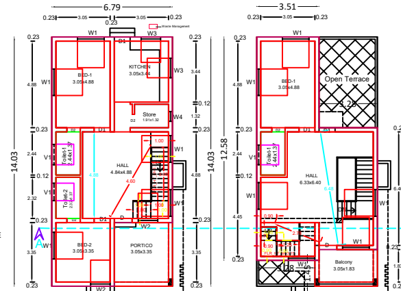
BLOCK-01 GROUND FLOOR PLAN
