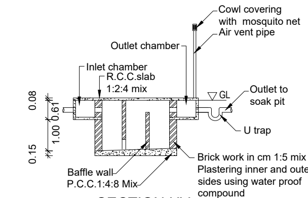
SECTION UV
