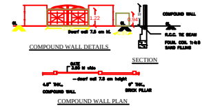
COMPOUND WALL PLAN
