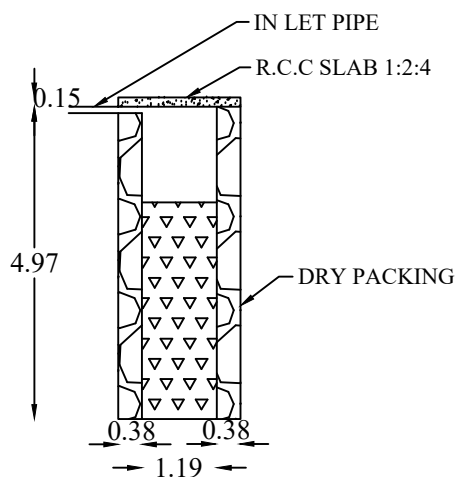
WASTE WATER TANK
