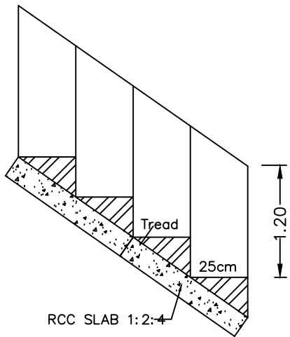
STAIR DETAILS
